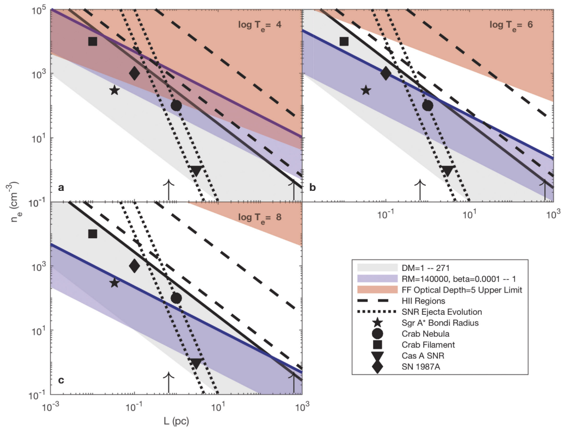
Extended Data Figure 6 | Physical constraints from source parameters. a–c, Parameter space for the electron density ( n_e ) and length scale ( L_{\text{RM}} ) of the Faraday region for three different temperature regimes, T_e = 10^4 K (a), 10^6 K (b) and 10^8 K (c). The shaded red region indicates the parameter space excluded because of optical depth considerations (optical depth from free–free absorption \tau_{\text{ff}} > 5 ). The solid black line indicates the maximum \text{DM}_{\text{host}} permitted, while the shaded grey region shows the dispersion measure down to 1 \text{ pc cm}^{-3} . The solid blue line denotes \text{RM}_{\text{src}} . The shaded blue region shows the range 10^{-4} \leq \beta \leq 1 . The intersection of grey and blue regions outside of the red region is physically permitted. The arrows indicate the upper limits on the sizes of the persistent source
