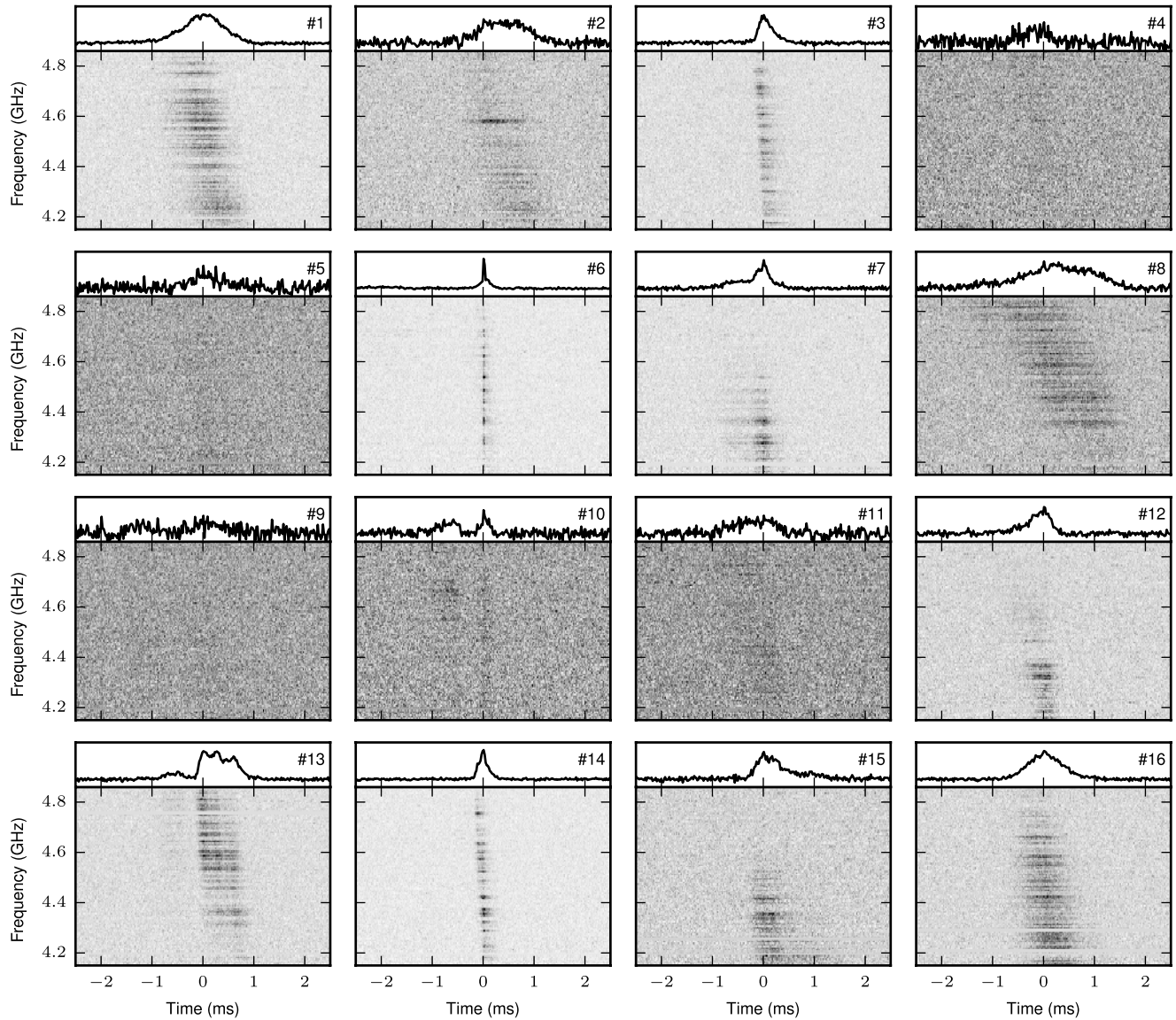
Extended Data Figure 1 | Pulse profiles and spectra of 16 Arcibo bursts. The bursts are dedispersed to DM = 559.7 \text{ pc cm}^{-3} (which minimizes the width of burst 6) and plotted with time and frequency resolutions of 20.48 \mu\text{s} and 6.24 \text{ MHz} , respectively.
